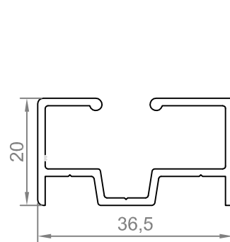
MONTANT ALUMINIUM
