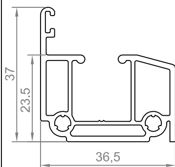
RAIL PVC
