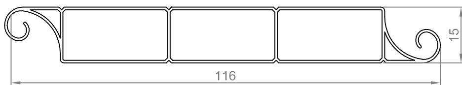
LAME PVC 116
