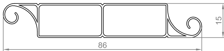
LAME PVC 86
