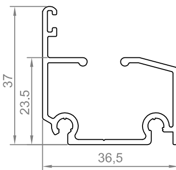
RAIL ALUMINIUM
