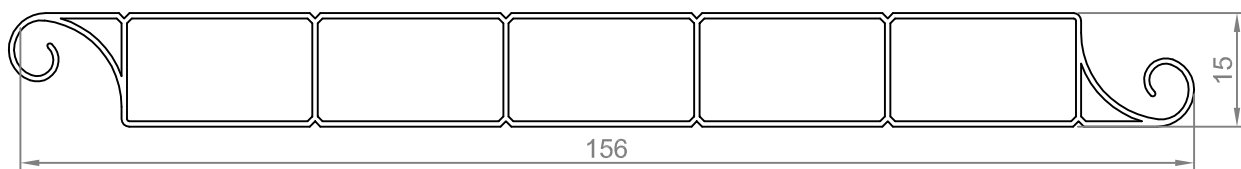
LAME PVC 156
